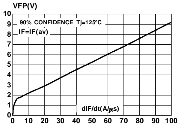
Fig 18 : Transient peak forward voltage versus dI_F/dt
