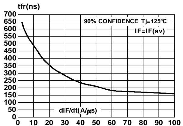
Fig 19 : Forward recovery time versus dI_F/dt
