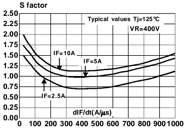
Fig 16 : Softness factor (tb/ta) versus dI_F/dt
