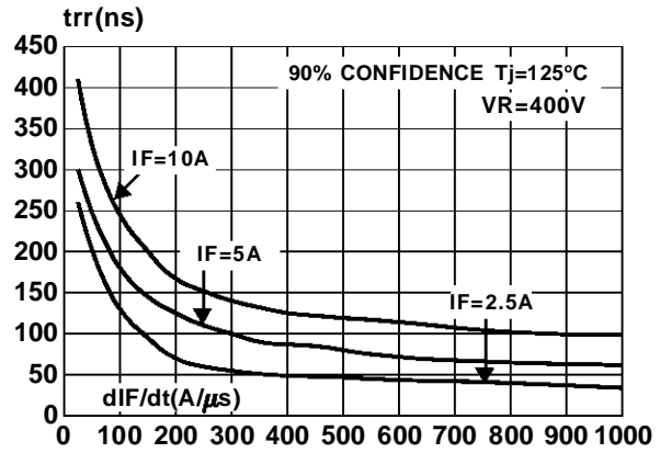
Fig 15 : Reverse recovery time versus dI_F/dt
