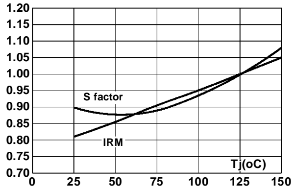
Fig 17 : Relative variation of dynamic parameters versus junction temperature (Reference T_j=125^\circ C )
