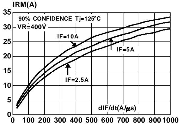
Fig 14 : Peak reverse recovery current versus dI_F/dt
